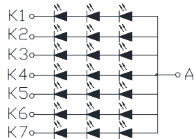
BACKLIGHT CIRCUIT DIAGRAM 9.6V(typ.)@140mA(constant)
